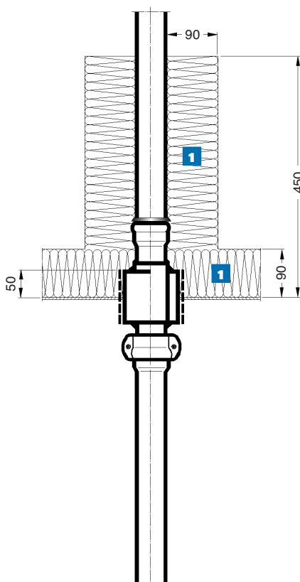
Bulkhead Penetration DN 40 Form T1S
