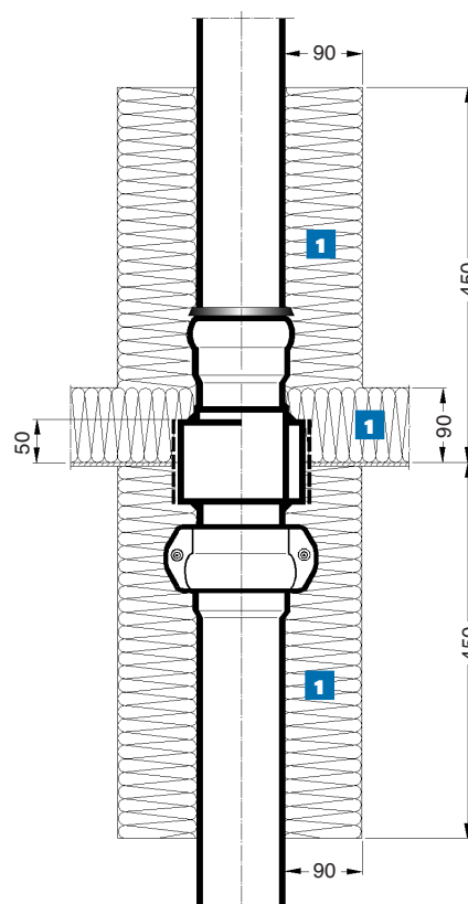
Bulkhead Penetration DN 50 - 200 Form T1S
