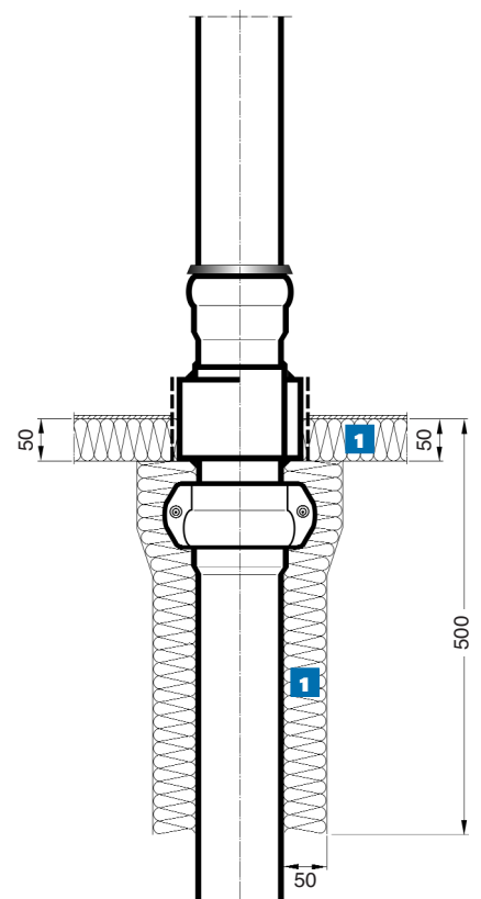
Deck Penetration DN 40 - 200 Form T1S
