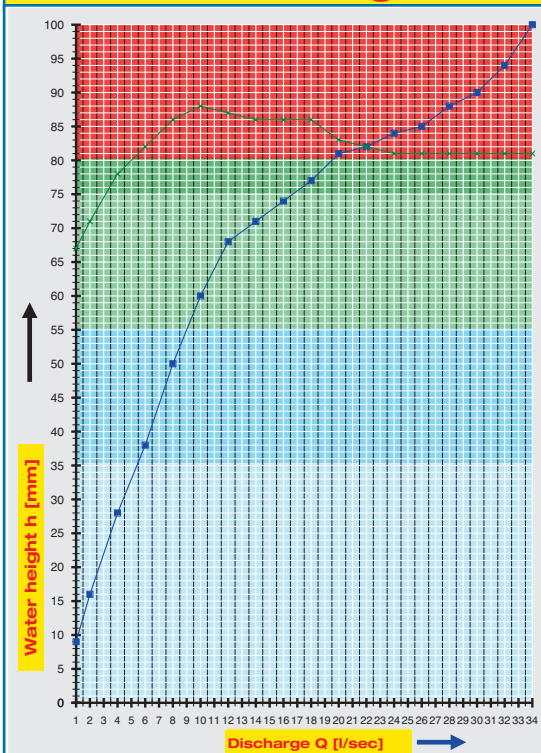
hQ - Head-Discharge curve
