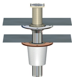
Strainer unit, Series F No. 15081X
