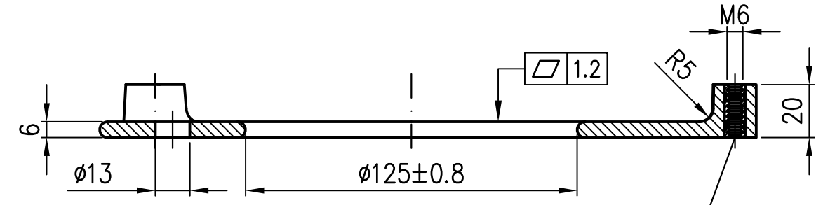
Buchse M6x20, Messing
